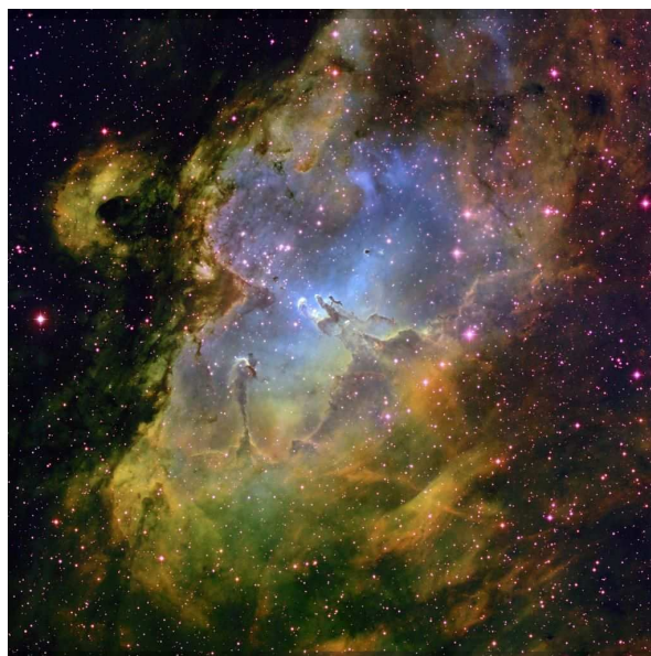
Hubble-eagle-nebula-wide-field
